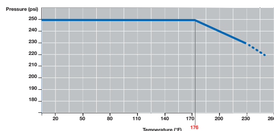
Pressure graph as a function of temperature
