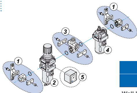
Two-block filter-regulator
