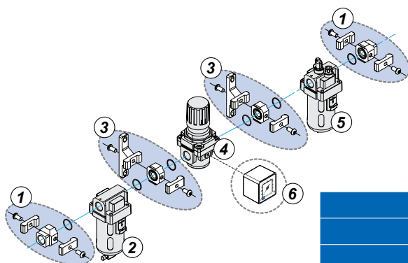
Three-block filter-regulator
